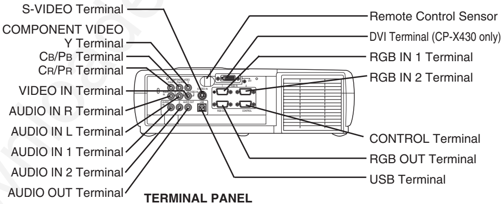
TERMINAL PANEL
