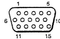
D-sub 15pin shrink terminal (Male)
