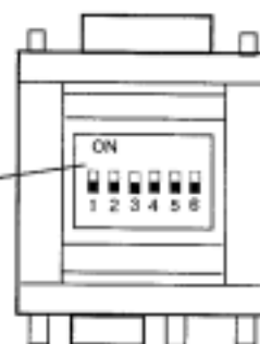
VGA/MAC ADAPTER
