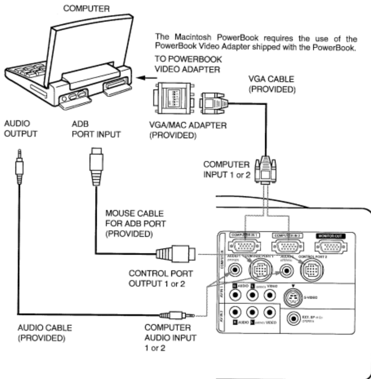
VGA/MAC ADAPTER
